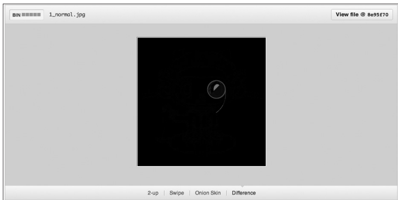
图 7.7 Difference
